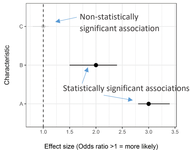
Figure 1 - example results from a logistic regression
