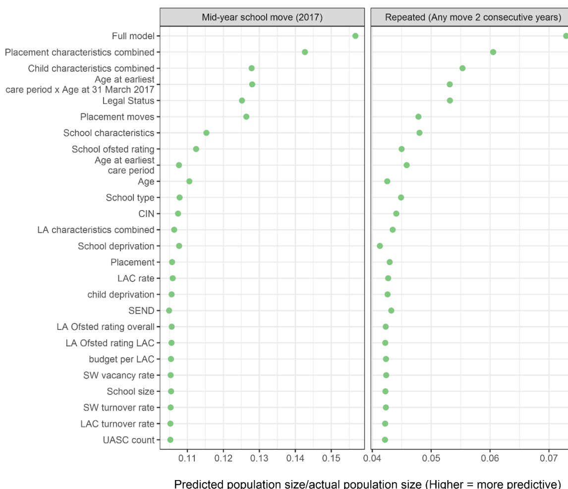
Figure 40 - Ratios of predicted population size to actual population size (variable explanatory power) for each variable tested, selected combinations of variables and all variables together. Higher values (points further to the right) indicate more predictive variables/groups of variables
