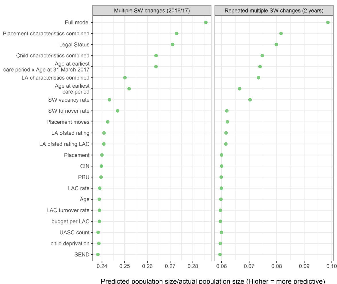
Figure 53 - Ratios of predicted population size to actual population size (variable importance) for each variable tested, selected combinations of variables and all variables together. Higher values (points further to the right) indicate more predictive variables/groups of variables. For comparability, all models are fitted on children from the 78 local authorities matched with the School Census.
